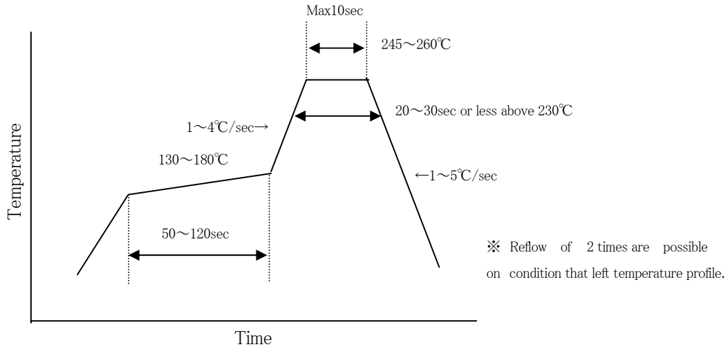
Temperature Profile of IR Reflow(After reflow, don't be cool sudden decrease.)
