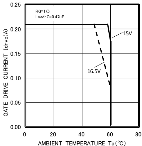
I_{drive} - T_a CHARACTERISTICS (MAXIMUM RATING)
