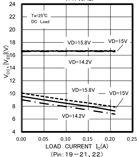
V_{CC}, |V_{EE}| - I_o CHARACTERISTICS (TYPICAL)
