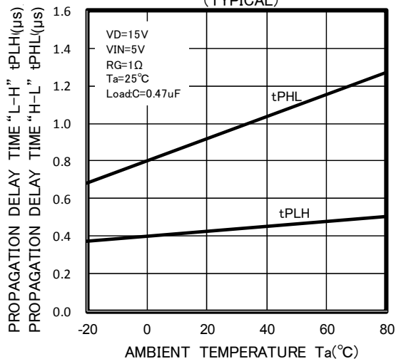
t_{PLH}, t_{PHL} - T_a CHARACTERISTICS (TYPICAL)
