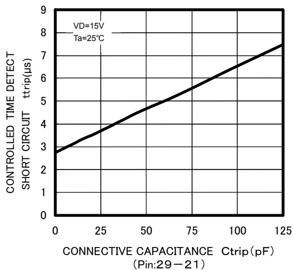
t_{trip} - C_{trip} CHARACTERISTICS (TYPICAL)
