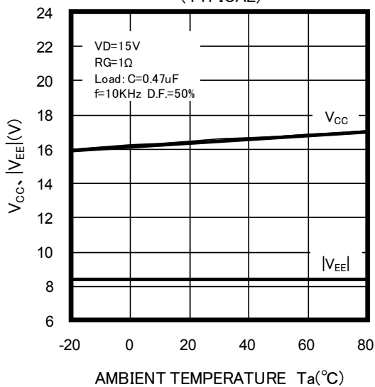
V_{CC}, |V_{EE}| - T_a CHARACTERISTICS (TYPICAL)
