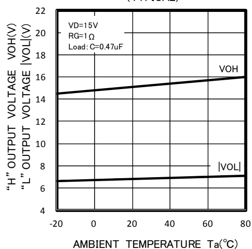
VOH,|VOL|- T_a CHARACTERISTICS (TYPICAL)
