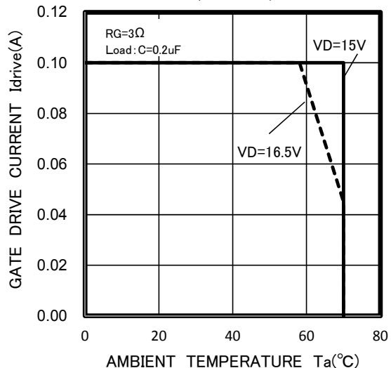
I_{drive} - T_a CHARACTERISTICS (TYPICAL)
