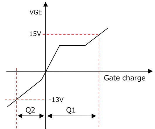
Gate charge characteristic of IGBT
