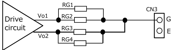
Layout pattern connection on substrate
