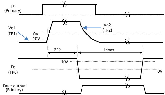
Operation of short circuit protection
