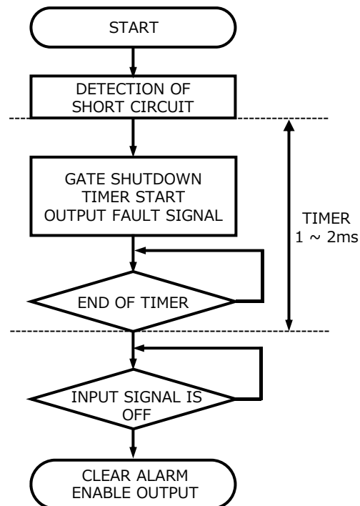
OPERATION FLOW ON DETECTING SHORT CIRCUIT
