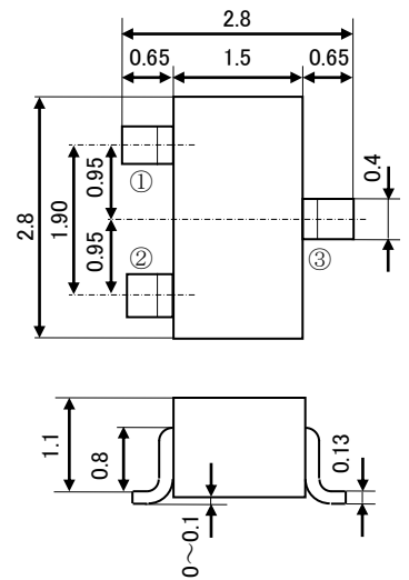
RT1P441C
