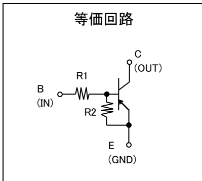
RT1P441U
