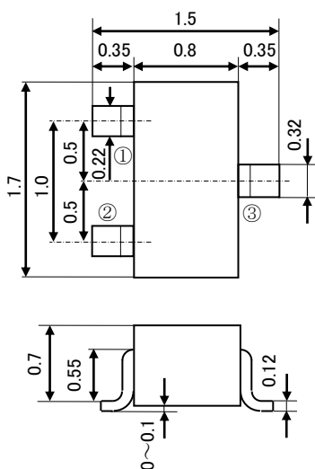
RT1P441U
