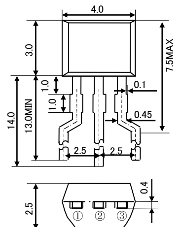
RT1P441S
