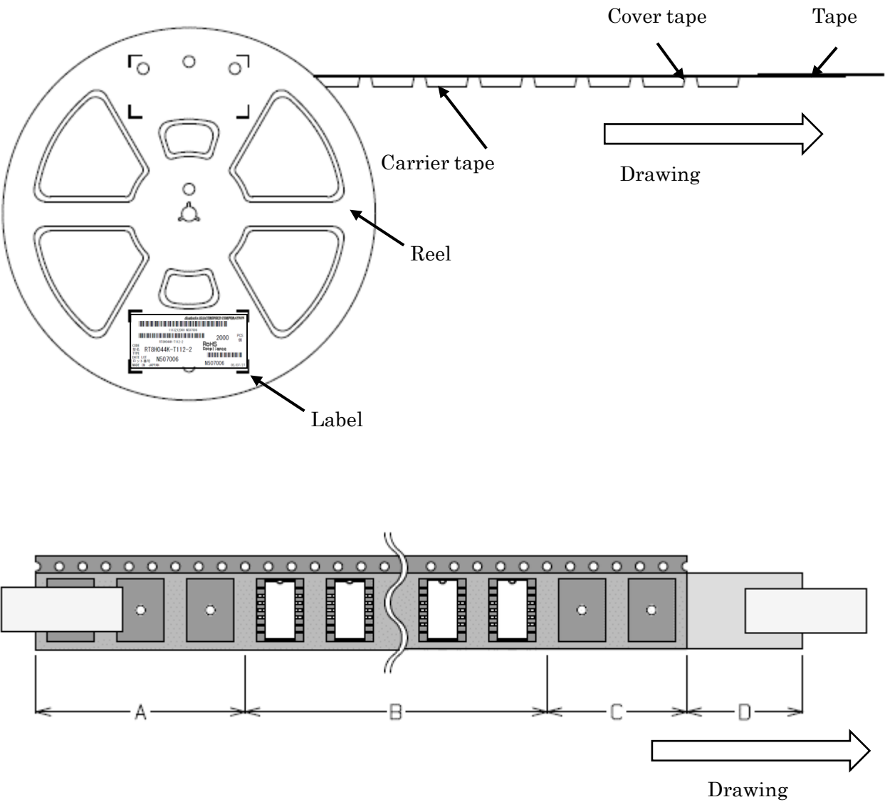
figure3. .Leader and trailer
