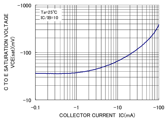
COLLECTOR EMITTER SATURATION VOLTAGE VS. COLLECTOR CURRENT
