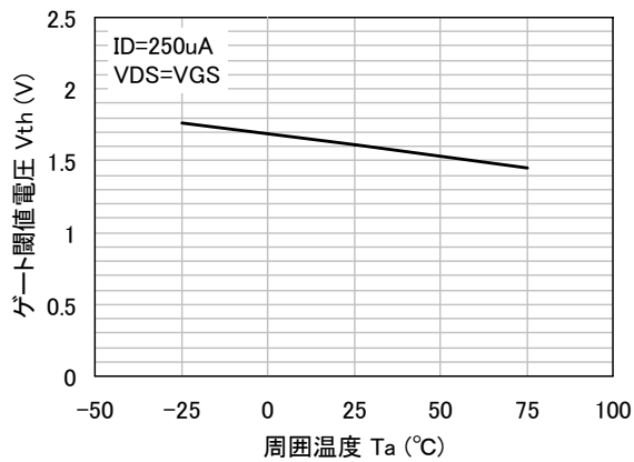
Vth - Ta
