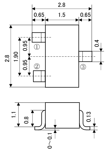
RT1N231C
