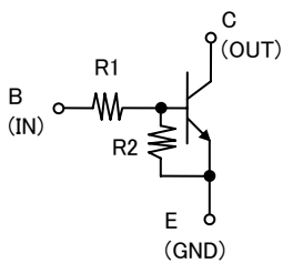
RT1N231U
