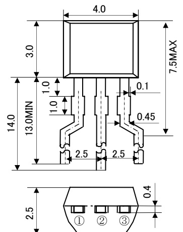
RT1N231S
