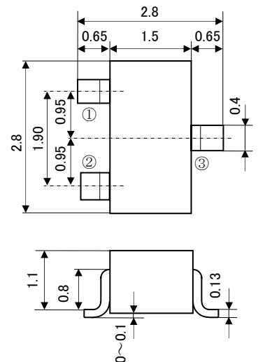
RT1N241C
