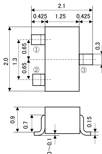
RT1N241M
