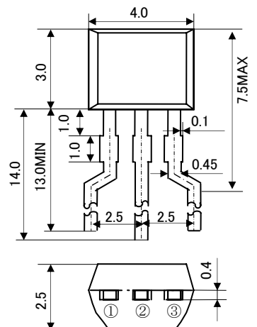
RT1N241S
