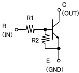
RT1N241U
