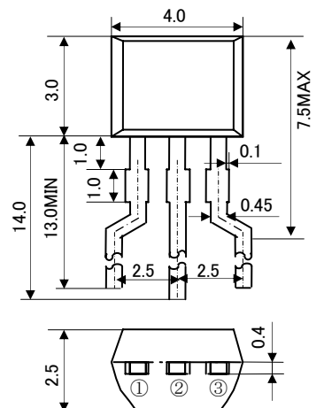
RT1P44BS
