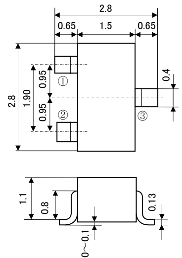
RT1P44BC
