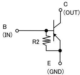
RT1P44BU
