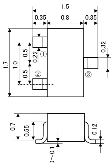
RT1P44BU
