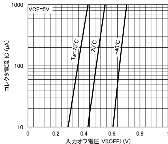
IC-VI(OFF)
