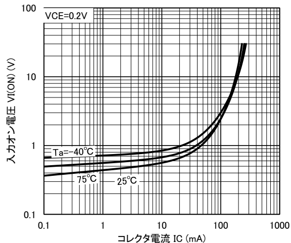
VI(ON)-IC
